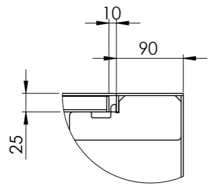
DETAIL D SCALE 1 : 5
