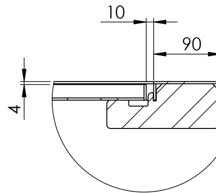
DETAIL E SCALE 1 : 5
